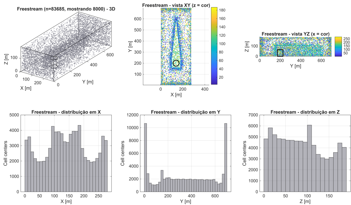
FIGURA 3: Freestream (n=83685, 39.3% do total)
